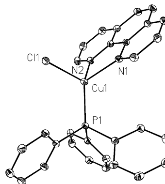
Figure 5. ORTEP drawing of [(\text{Ph}_3\text{P})\text{Cu}(\text{phen})\text{Cl}] \cdot \text{C}_2\text{H}_4\text{Cl}_2 ( 6 · \text{C}_2\text{H}_4\text{Cl}_2 ) with the cocrystallized molecule of 1,2-dichloroethane and all H atoms omitted for clarity and thermal ellipsoids drawn at the 50% probability level.
